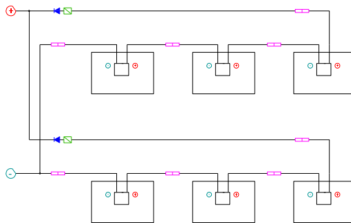
Series Wiring and Parallel Wiring
