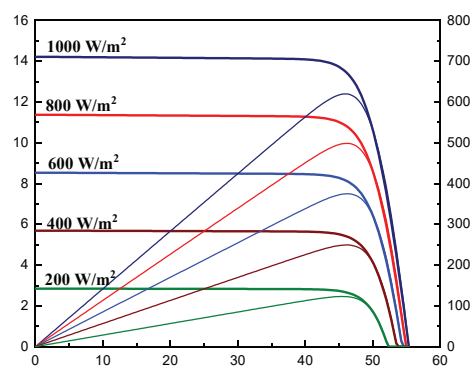
Current - Voltage & Power - Voltage Curve (TT620-156TN10)
