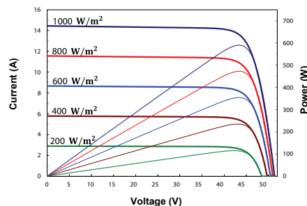
Current - Voltage & Power - Voltage Curve (CWT595 - 144TNCK10)
