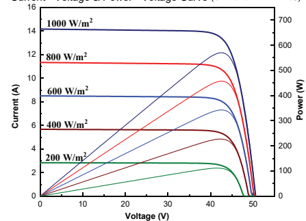
Current - Voltage & Power - Voltage Curve (CWT570 - 144TNB10)
