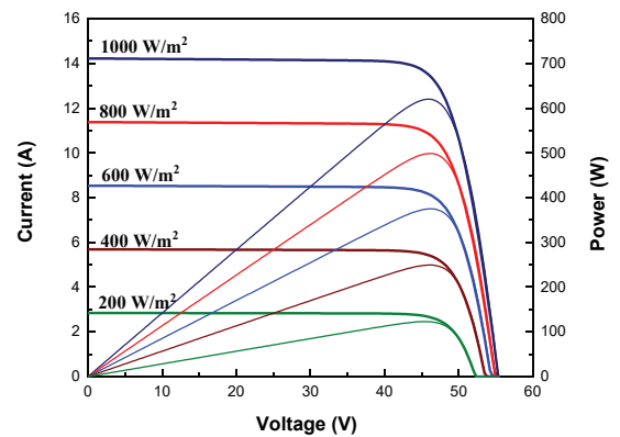
Current - Voltage & Power - Voltage Curve (CWT620-156TN10)
